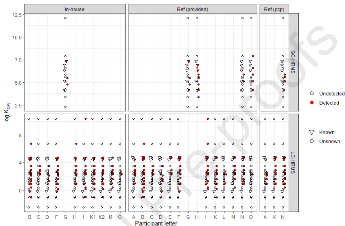
Fig. 4. Predicted \log K_{OW} values of spiked compounds. Log K_{OW} values of spiked compounds predicted by participants ( n = 16 , code A-P) using EPI Suite 4.0, along with indication of positive (red) or negative (white) detection. Unknown compounds (spiked compounds whose identity was not disclosed) are indicated with a circle, while known compounds (spiked compounds whose identity was revealed to the participants) are marked with a triangle. The compounds are grouped according to sample preparation method (Ref (provided) = provided reference extract, Ref (pcp) = extract prepared with the reference method by the participant, in-house = extract prepared with the participant's in-house protocol) and method of analysis (LC-HRMS, or GC-HRMS). If the same laboratory analysed extracts from several in-house sample preparation protocols, these were allocated sequential numbers following the laboratory code letter (e.g. K1, K2).
