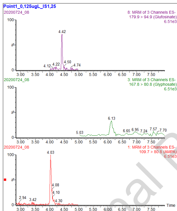
Figure 1. MRM chromatogram of a calibration solution containing AMPA, glufosinate, and glyphosate at the limit of quantification (LOQ) of 0.125 \mu\text{g/L}
