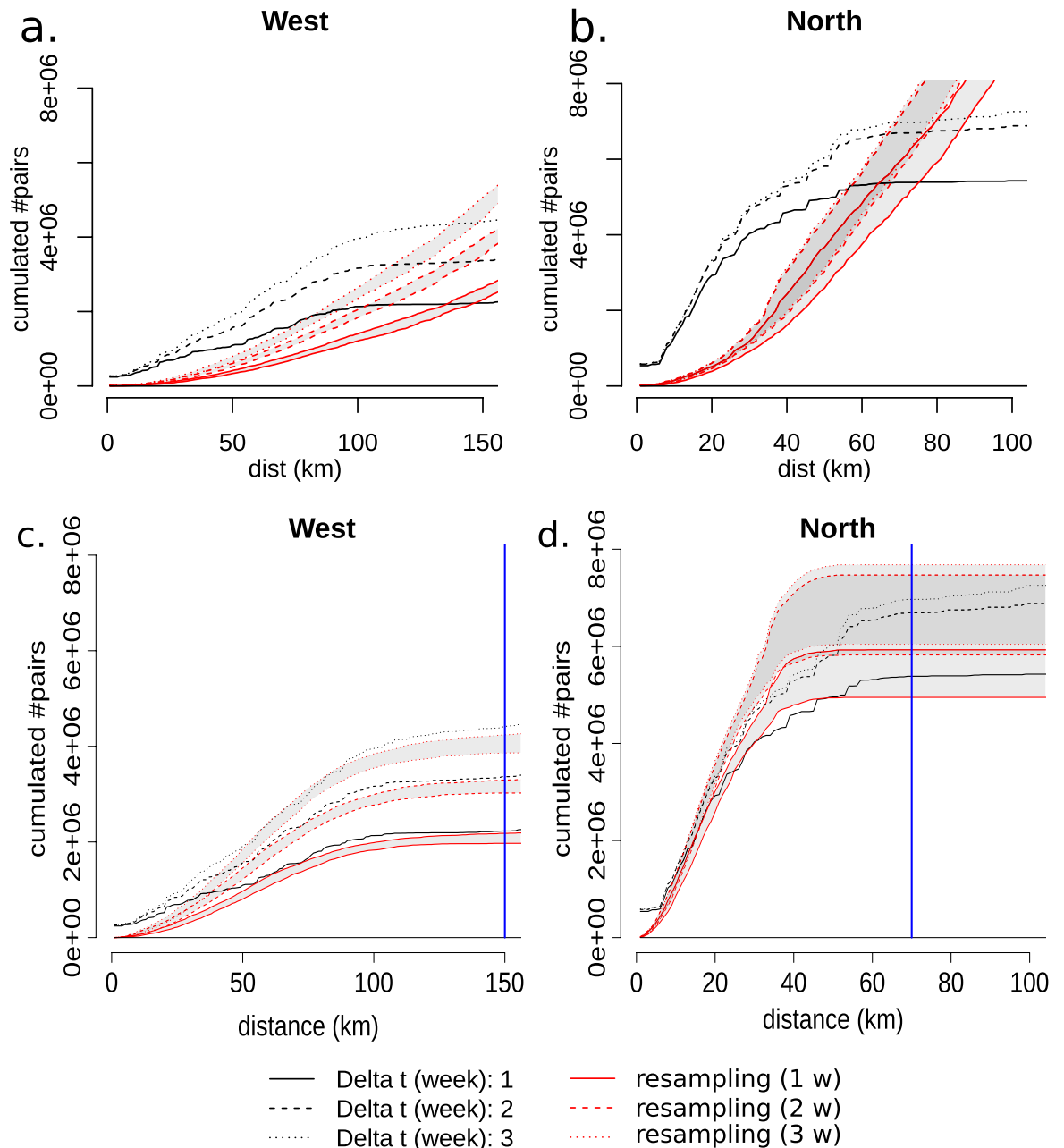
Figure 2. K-Ripley analysis (Null-model) of the meningitis epidemic events for the Western and Northern subregions, in 13 health districts, Burkina Faso, 2004–2014. (a,c) Western subregion: Hauts-Bassin region and Dédougou district. (b,d) Northern subregion: Nord region. Boulsa district was excluded from this analysis due to the low number of epidemic events detected. Black lines, number of pairs of epidemic HC that are closer than a given spatio-temporal horizon on the x-axis: 1, 2 and 3 weeks for spatial horizons ranging from 0 to 100/150 km. Red lines, 5th and 95th percentile of resampled distributions over 20 simulations of the generative model. (a, b) Null model without clustering or correlation. (c,d) Model incorporating both spatial clustering and temporal correlation blue line: range over which the observed K-Ripley is higher than the null models (Western 0–150 km, Northern: 0–70 km).
