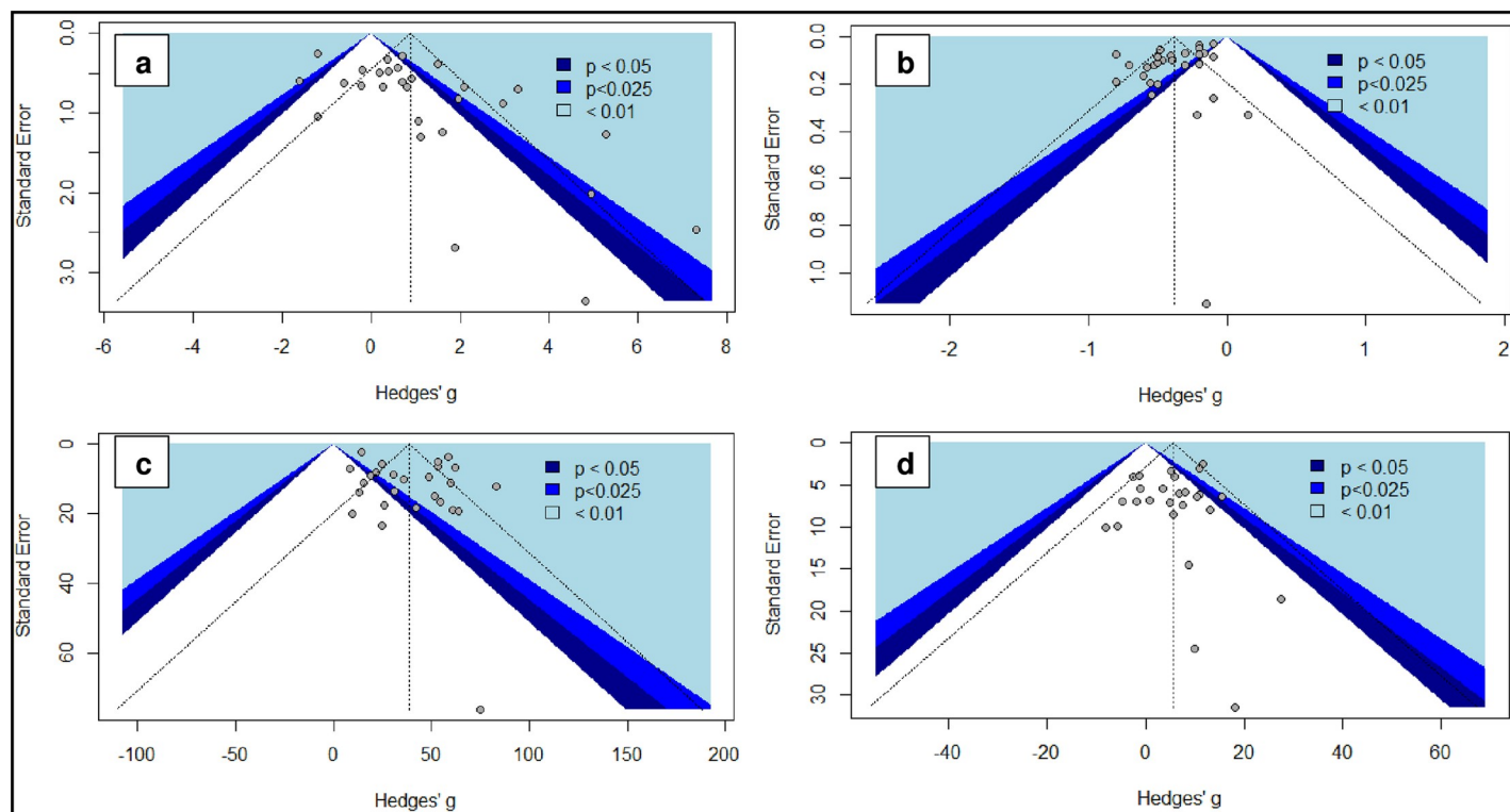
Fig 3. Funnel plots. a: White cell count, Egger's test, p = 0.004 ; b: Lymphocytes, Egger's test, p = 0.005 ; c: C-Reactive protein, Egger's test, p = 0.155 ; d: Creatinine, Egger's test, p = 0.415 .
