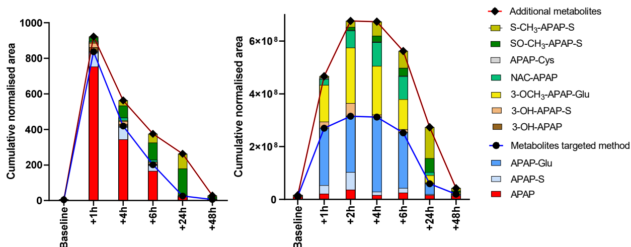
Fig. 3. Analytical responses (represented as cumulative normalised peak areas) of APAP metabolites classically used for targeted methods (i.e., free APAP, APAP-Glu and APAP-S) and the other metabolites detected using the non-targeted analyses in blood (A) and urine (B) of the 4 men. APAP and its metabolites were manually re-integrated using the Sciex OS Analytics tool. The integrated peak area of individual markers was normalized to APAP-d4 for plasma or with a corrective factor based on the total peak area for urine.
