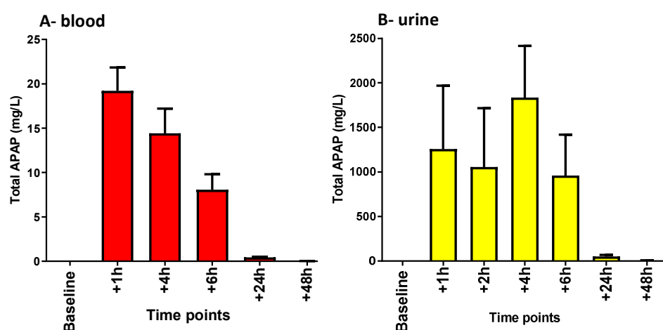
Fig. 1. “Total” APAP concentrations (free APAP, APAP glucuronide and APAP sulfate) after enzymatic deconjugation using LC-MS/MS in (A) blood plasma (mg/L, mean \pm SEM) and (B) urine (mg/L, mean \pm SEM) of
