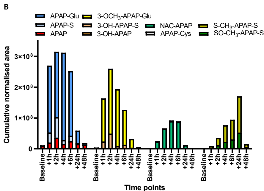
Fig. 4. Kinetics of formation of free APAP, phase II metabolites (APAP-Glu and APAP-S), catechol metabolites (3-OCH 3 -APAP-Glu, OH-APAP-S and OH-APAP), glutathione derived metabolites (NAC-APAP and APAP-Cys) and thiomethyl metabolites (S-CH 3 -APAP-S and SO-CH 3 -APAP-S) detected using the non-targeted screening based on UHPLC-ESI-QTOF-MS analyses in (A) blood plasma and (B) urine of the 4 men before intake and at different time points after intake. No significant shift (i.e. below 20%) in analytical sensitivity was observed during the batch to make this time point comparison for individual metabolites. APAP and its metabolites were manually
