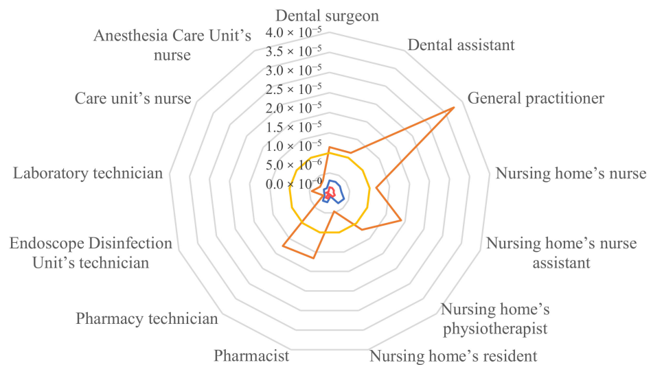
Figure 2. Excess lifetime cancer risks of benzene (blue), formaldehyde (orange) and acetaldehyde (red) against the acceptability threshold (yellow).
