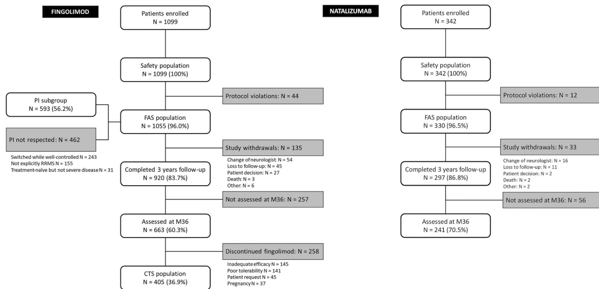
Fig. 1 Patient disposition. FAS full analysis set, CTS continuous treatment set, PI prescribing information compliant, RRMS relapsing–remitting multiple sclerosis. Percentages are calculated with respect to the number of
