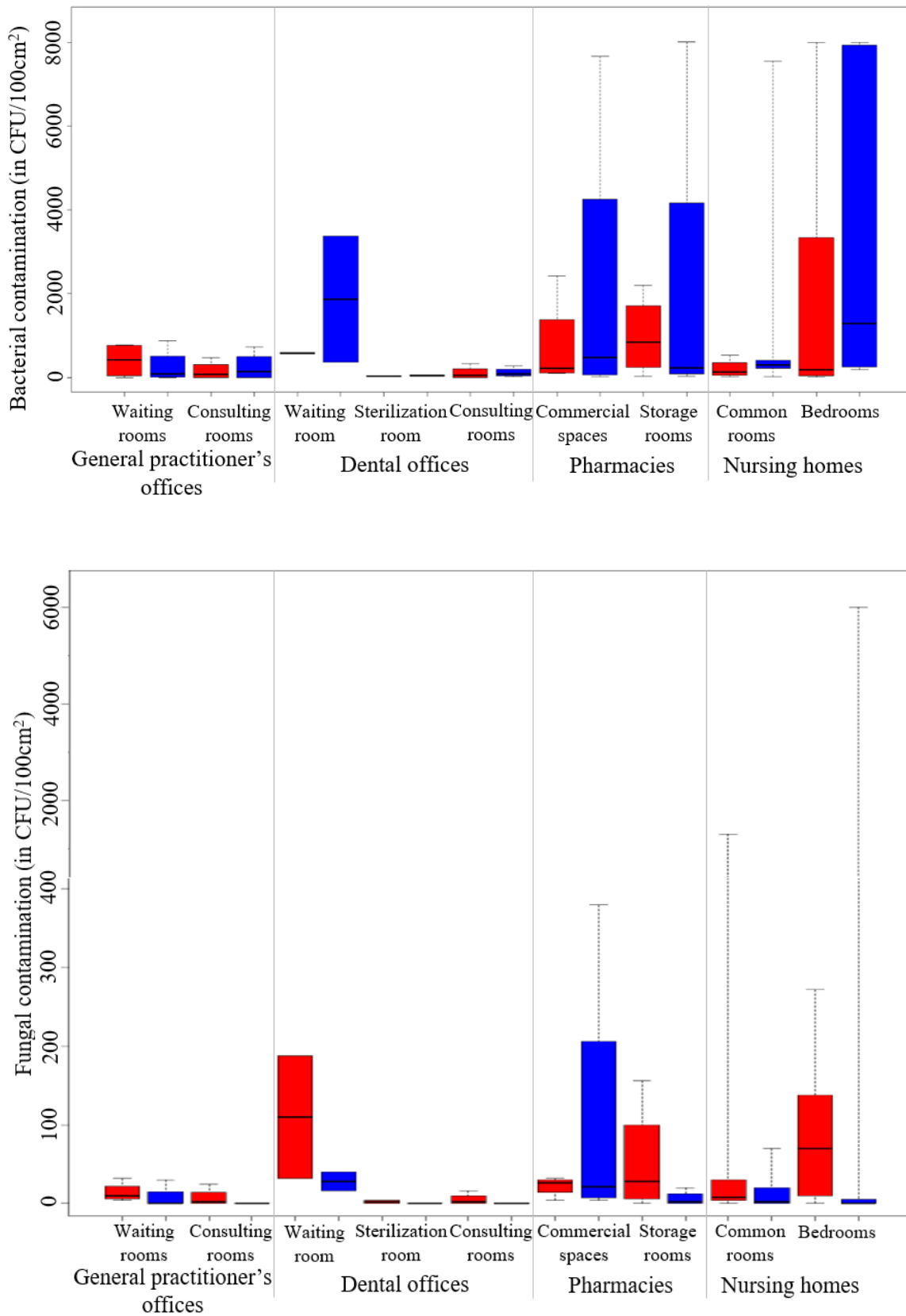
Figure 5. Bacterial and fungal contaminations on surfaces (CFU/100 cm 2 ) in each sampled room of healthcare and care facilities during summer (red) and winter (blue).
