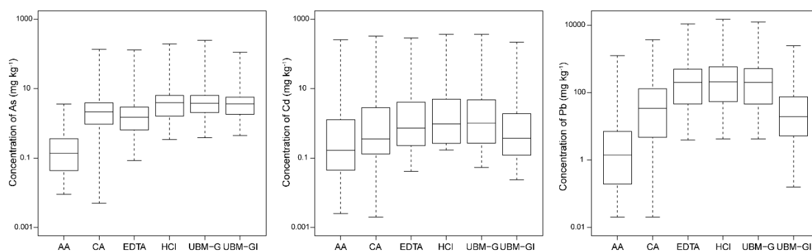
Figure 1. Boxplots of metal(loid)s concentrations extracted by acetic acid (AA), citric acid (CA), EDTA, HCl, and UBM in the gastric (UBM-G) and gastrointestinal (UBM-GI) phases ( n = 201 ; expressed in mg kg -1 ).
