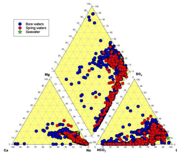
Fig. 2. Piper diagram
